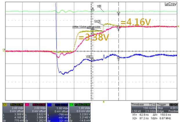
Figure 15. V_{OH} Level with C_{CP} = 2.2 nF (ch1: GATE pin; ch2: MOSFET Vgs; ch3 : VRAIN : ch4 : VDD)
