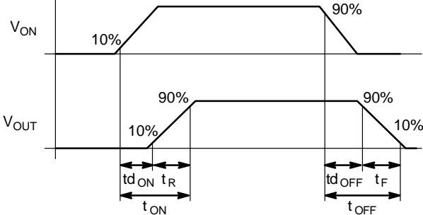
Figure 24. Timing Diagram
