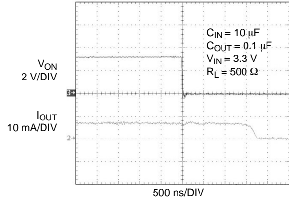
Figure 19. t_{dOFF} Response
