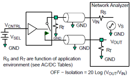
Figure 14. Channel Off Isolation
