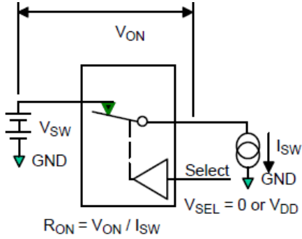
Figure 7. On Resistance
